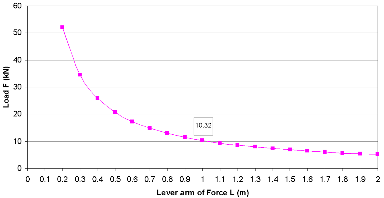
Load diagram for rotator CPR 5
